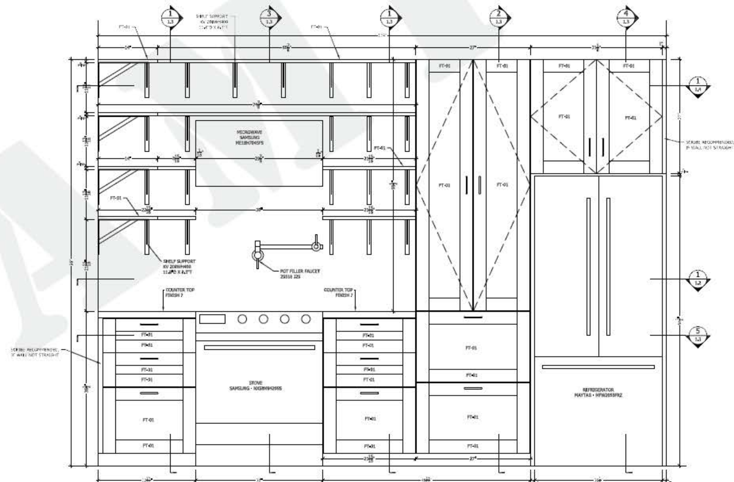
A ELEVATION KITCHEN SCALE: 1/4" = 1'-0" AND REV. 1 NONE
